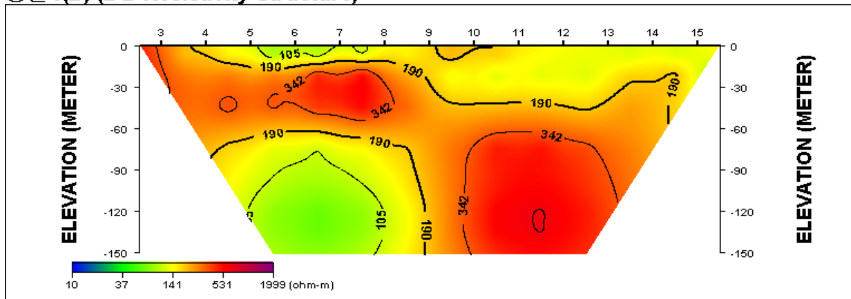
통산1(D) (2-D Resistivity Structure)
