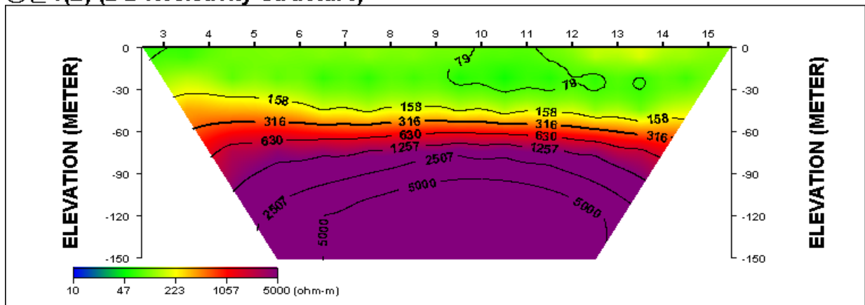
통산1(B) (2-D Resistivity Structure)
