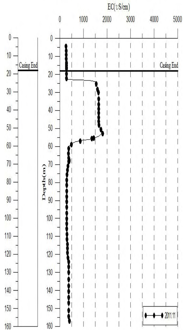
(b) EC검층
