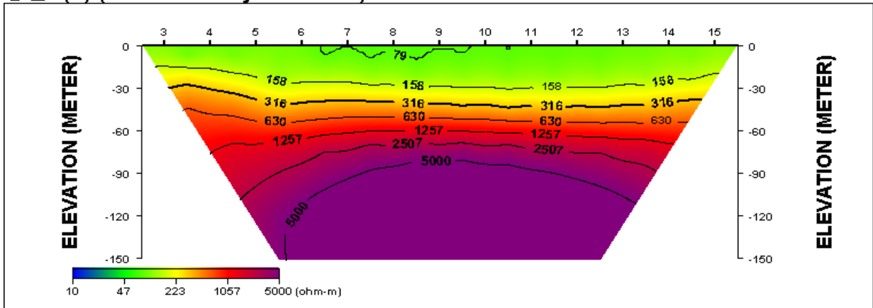
통산1(C) (2-D Resistivity Structure)
