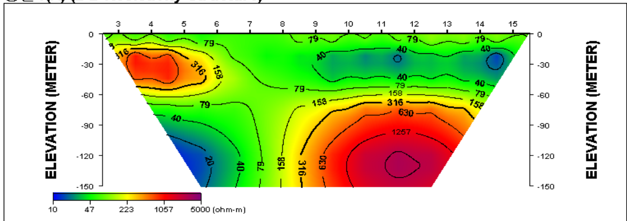
통산1(A) (2-D Resistivity Structure)
