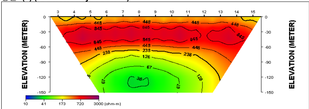
통산1(E) (2-D Resistivity Structure)
