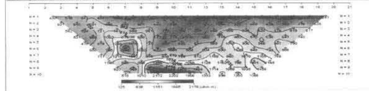
ES3-1 (2-D Resistivity Structure)
