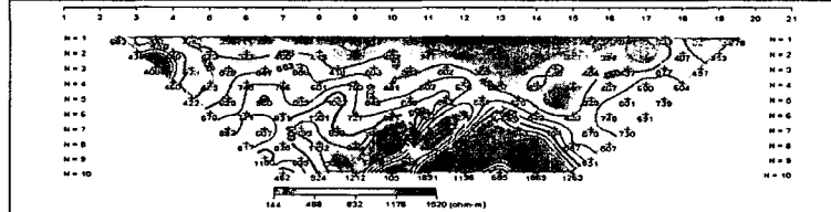
ES5-3 (Theoretical Data Pseudosection)
