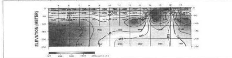
ES7-1 (2-D Resistivity Structure)
