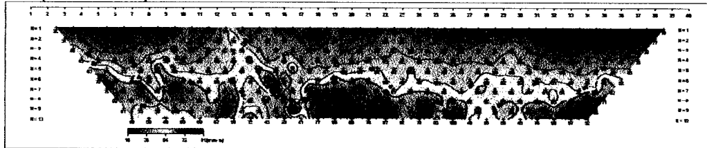
SN-DD01 (Theoretical Data Pseudocolor)
