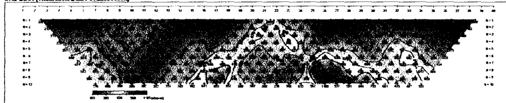
DKD-DD01 (2-D Resistivity Structure)
