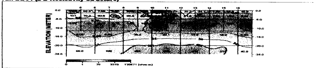
KM-DD01 (2-D Resistivity Structure)
