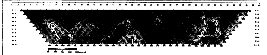
DC-DD01 (Theoretical Data Pseudocolor)
