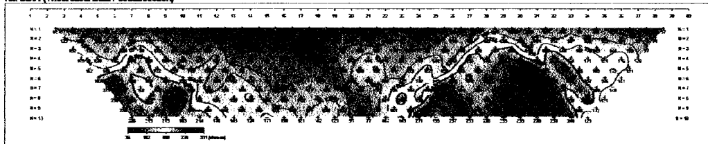
HM-DD01 (2-D Resistivity Structure)
