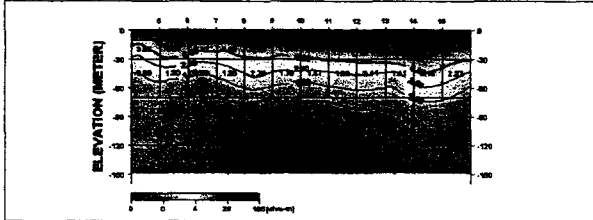
D-23 (2-D Resistivity Structure)
