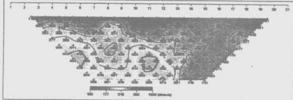
D-13 (2-D Resistivity Structure)
