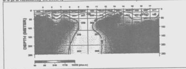
D-5 (2-D Resistivity Structure)
