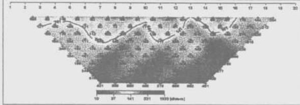
D-2 (2-D Resistivity Structure)
