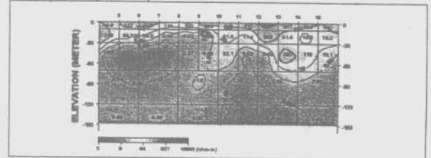
D-24 (2-D Resistivity Structure)
