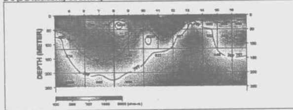
D-3 (2-D Resistivity Structure)
