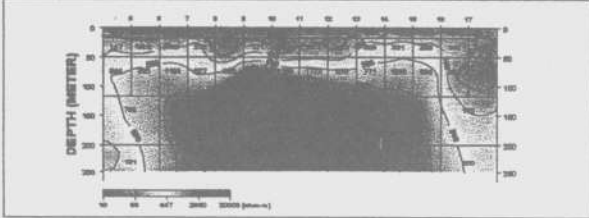
D-1 (2-D Resistivity Structure)
