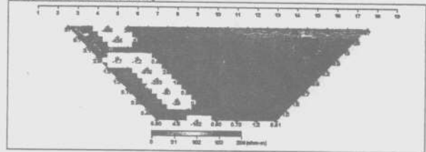
D-24 (Theoretical Data Pseudosection)
