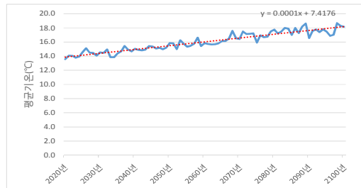
[RCP 8.5 평균기온]
