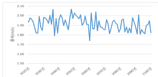
[RCP 8.5 풍속]
