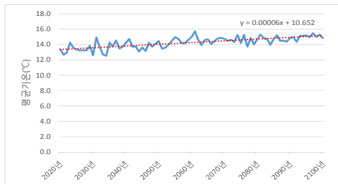
[RCP 4.5 평균기온]
