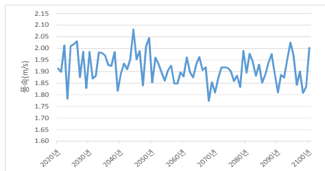
[RCP 4.5 풍속]
