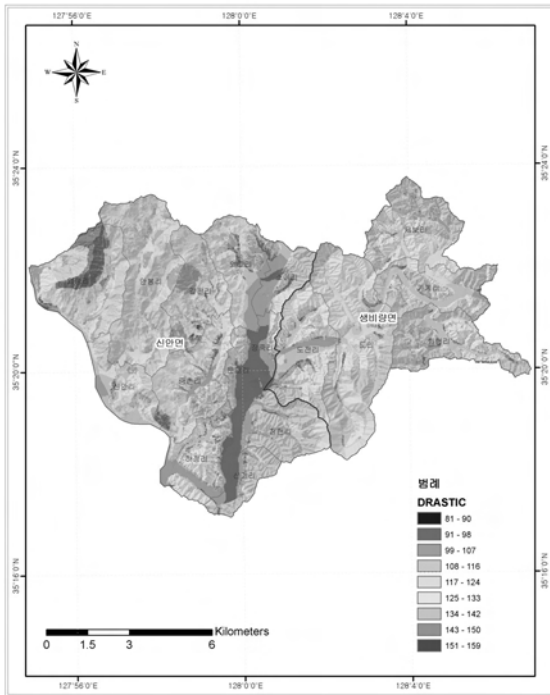
<DRASTIC Map>
