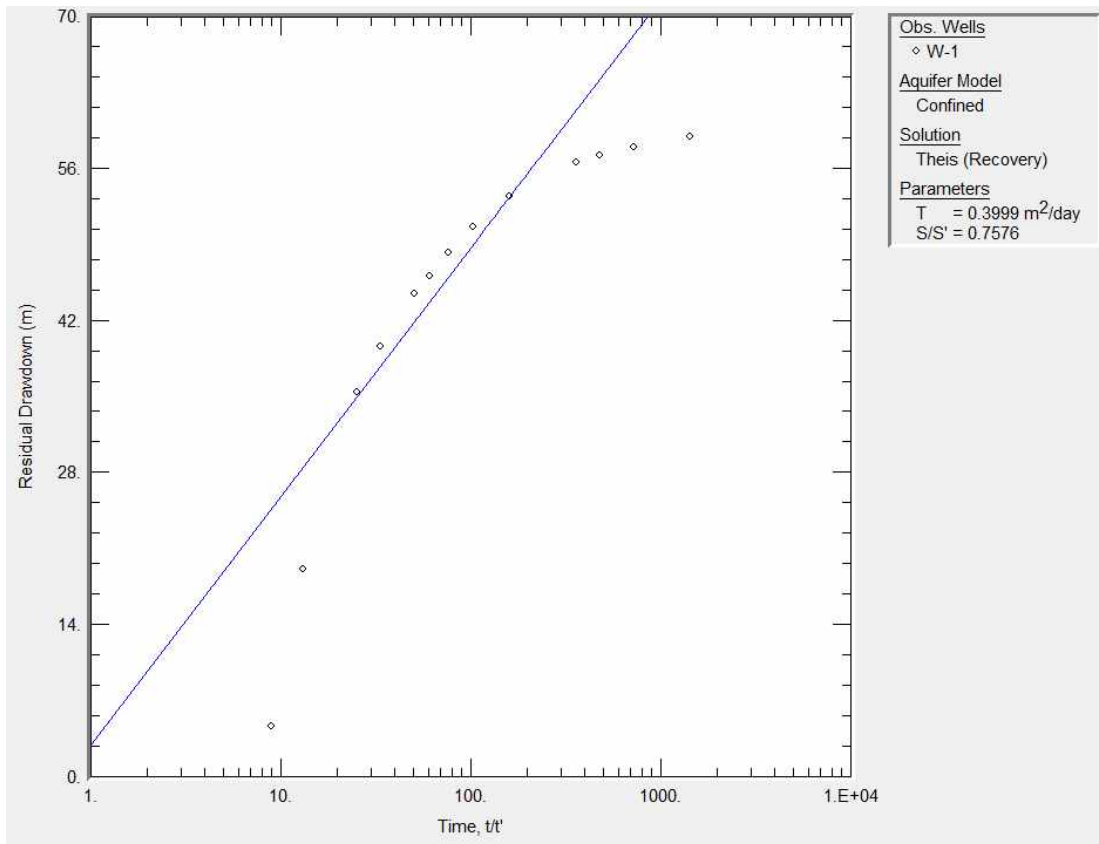
(b) Theis Recovery
