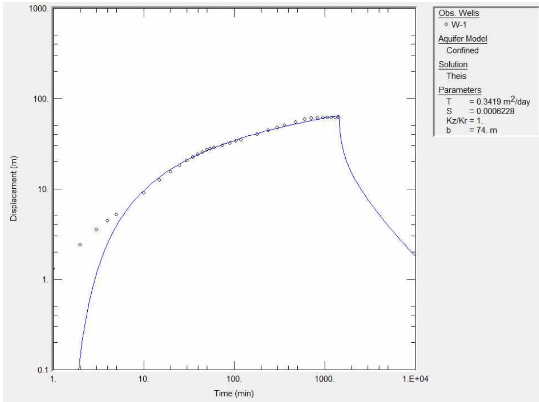
(a) Theis 해석법
