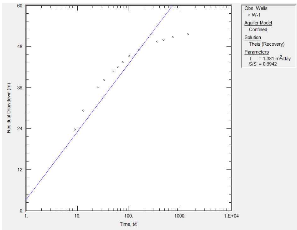
Theis Recovery
